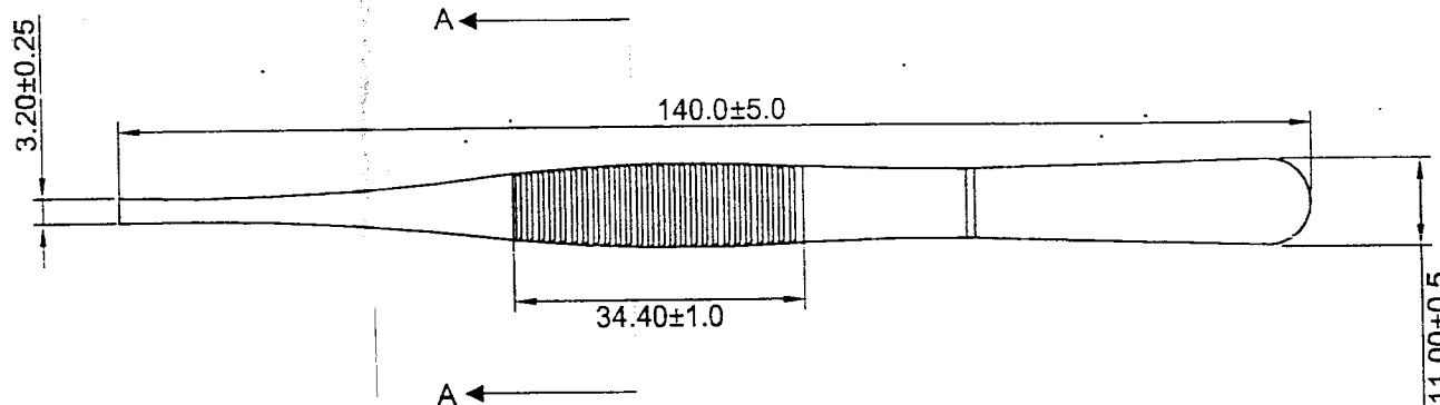
SIDE ELEVATION
